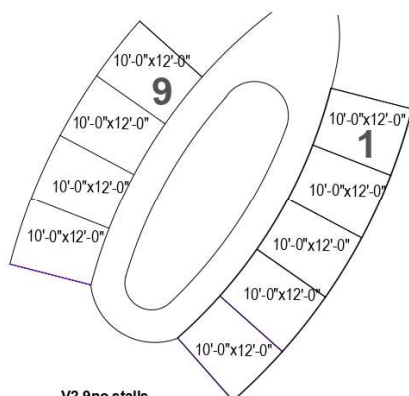
V2-9no.stalls (10'-0"X12'-0" each stall)ZONE 2
